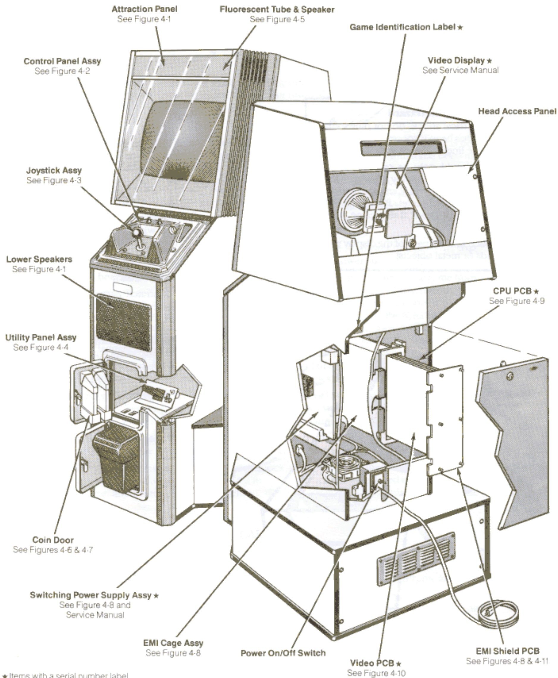
Figure 1-1 Game Overview
